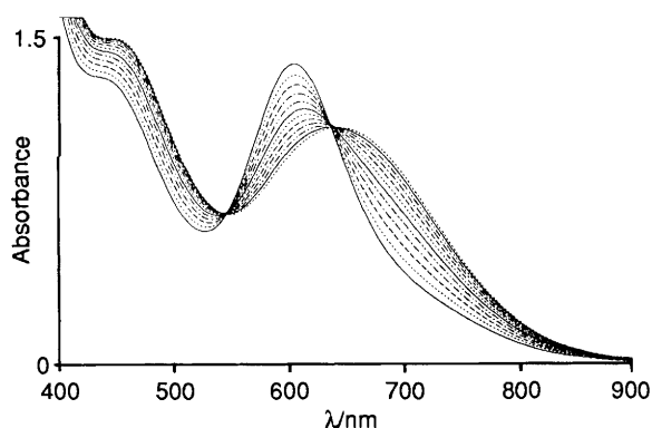
Fig. 1 Ultraviolet-visible spectral changes of a mixture of [\text{Fe}_3(\text{CO})_{12}] and \text{PPh}_3 in thf as a function of time; the time interval between spectroscopic measurements was 5 min. See run 1 in Table 1 for reaction conditions
