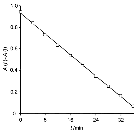
Fig. 2 The absorbance at 600 nm of a mixture of [\text{Fe}_3(\text{CO})_{12}] and \text{PPh}_3 in thf as a function of time; [\text{Fe}_3(\text{CO})_{12}] = 3.27 \times 10^{-3} , [\text{PPh}_3] = 6.07 \times 10^{-2} \text{ mol dm}^{-3} , 20 \pm 0.1^\circ\text{C} . See text for the definition of A(t) and A(f)
