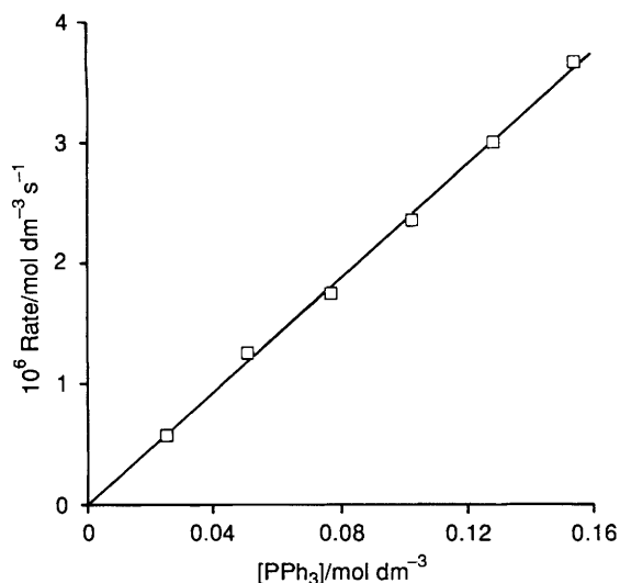
Fig. 3 Effect of the concentration of \text{PPh}_3 on the substitution rate of [\text{Fe}_3(\text{CO})_{12}]^- [ (2.49 \pm 0.05) \times 10^{-3} \text{ mol dm}^{-3} ]; runs 1–6
