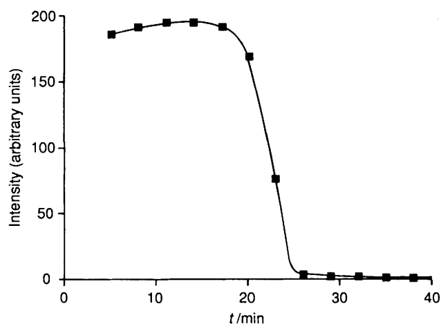
Fig. 4 The intensity of the [\text{Fe}_3(\text{CO})_{12}]^- signal as a function of time; [\text{Fe}_3(\text{CO})_{12}] = 5.02 \times 10^{-3} , [\text{PPh}_3] = 1.57 \times 10^{-1} \text{ mol dm}^{-3} , 20 \pm 0.5^\circ \text{C} . The concentration of [\text{Fe}_3(\text{CO})_{12}]^- at maximum intensity is estimated to be 1.5 \times 10^{-3} \text{ mol dm}^{-3}
